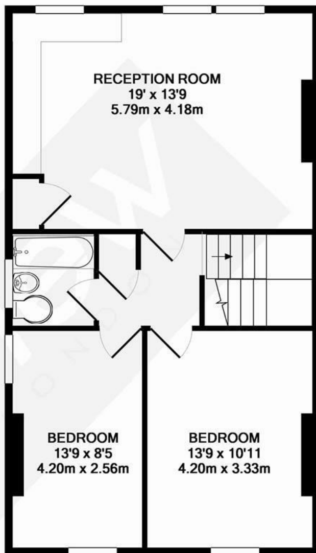
2ND FLOOR
